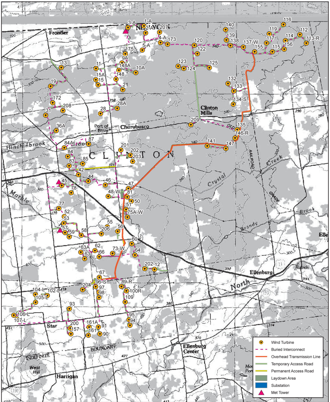
Figure 1: Project Layout (Revised)
