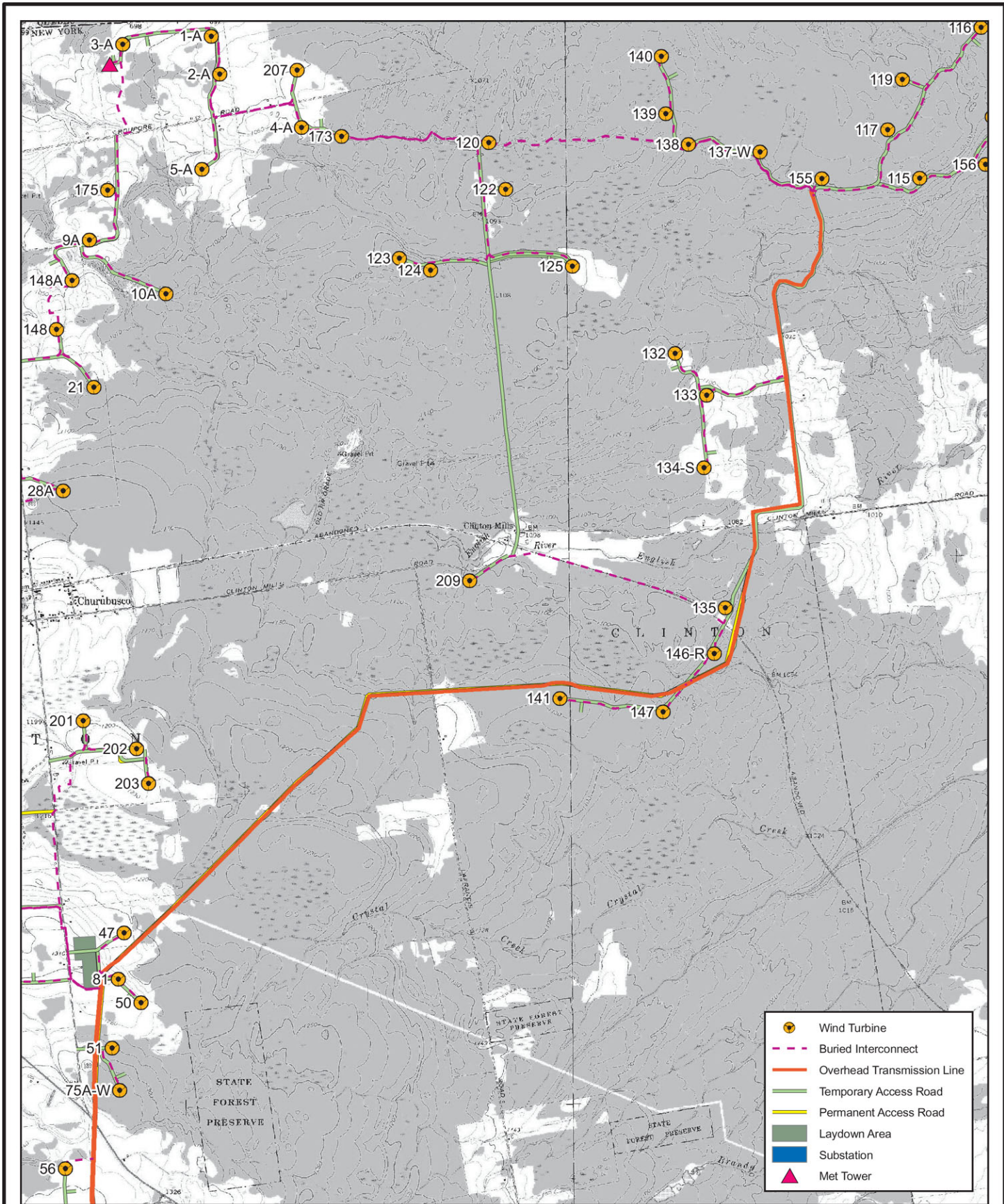
Figure 2: Access Road to Wind Turbine 209
