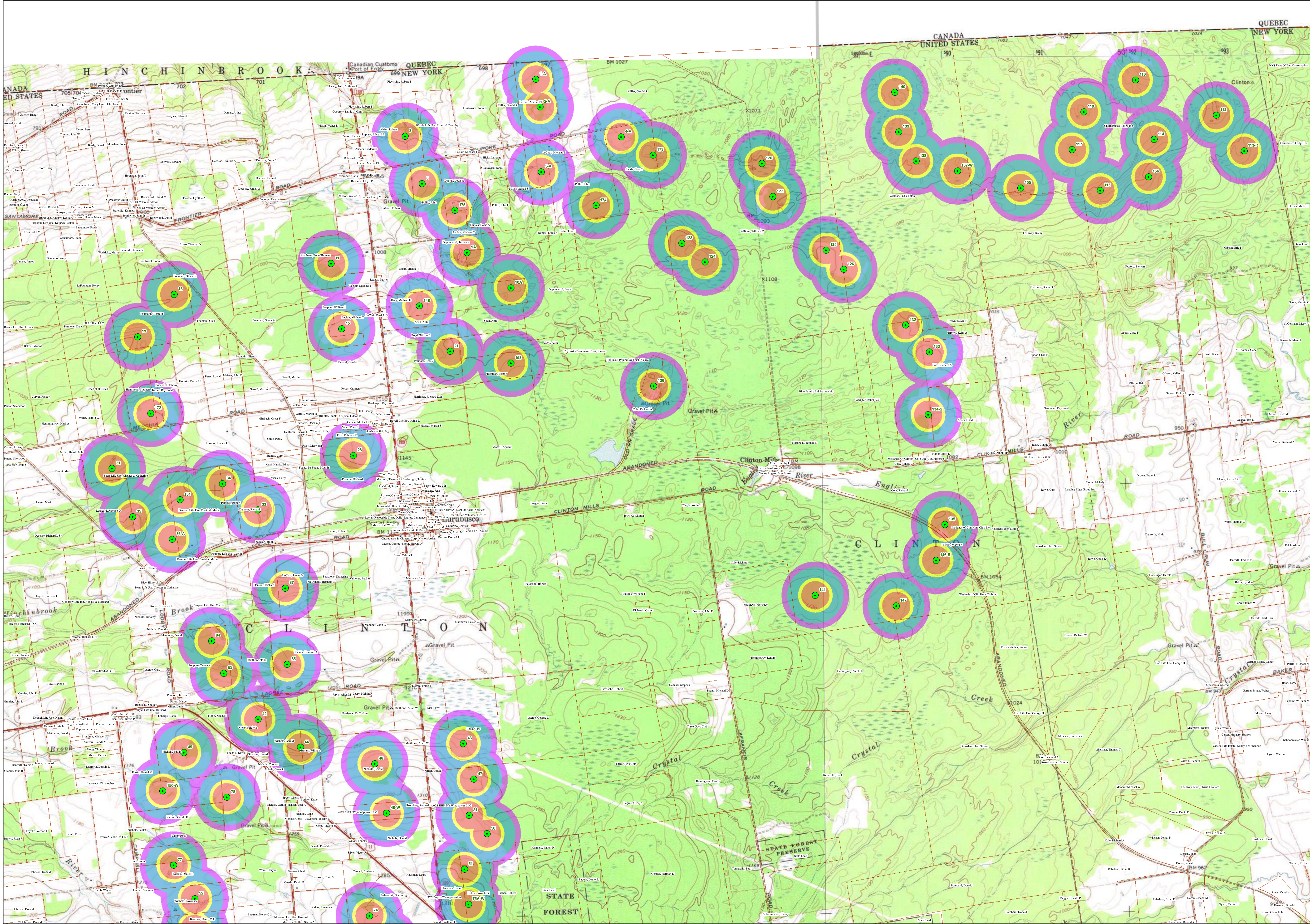
Exhibit 4R North Wind Turbine Setbacks Marble River Wind Clinton County, New York 4 January 2006
