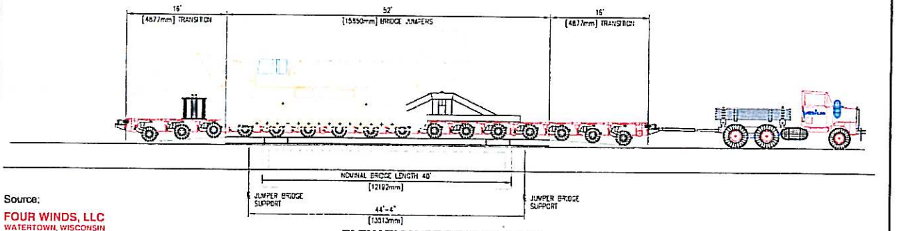
ELEVATION OF BRIDGE JUMP
